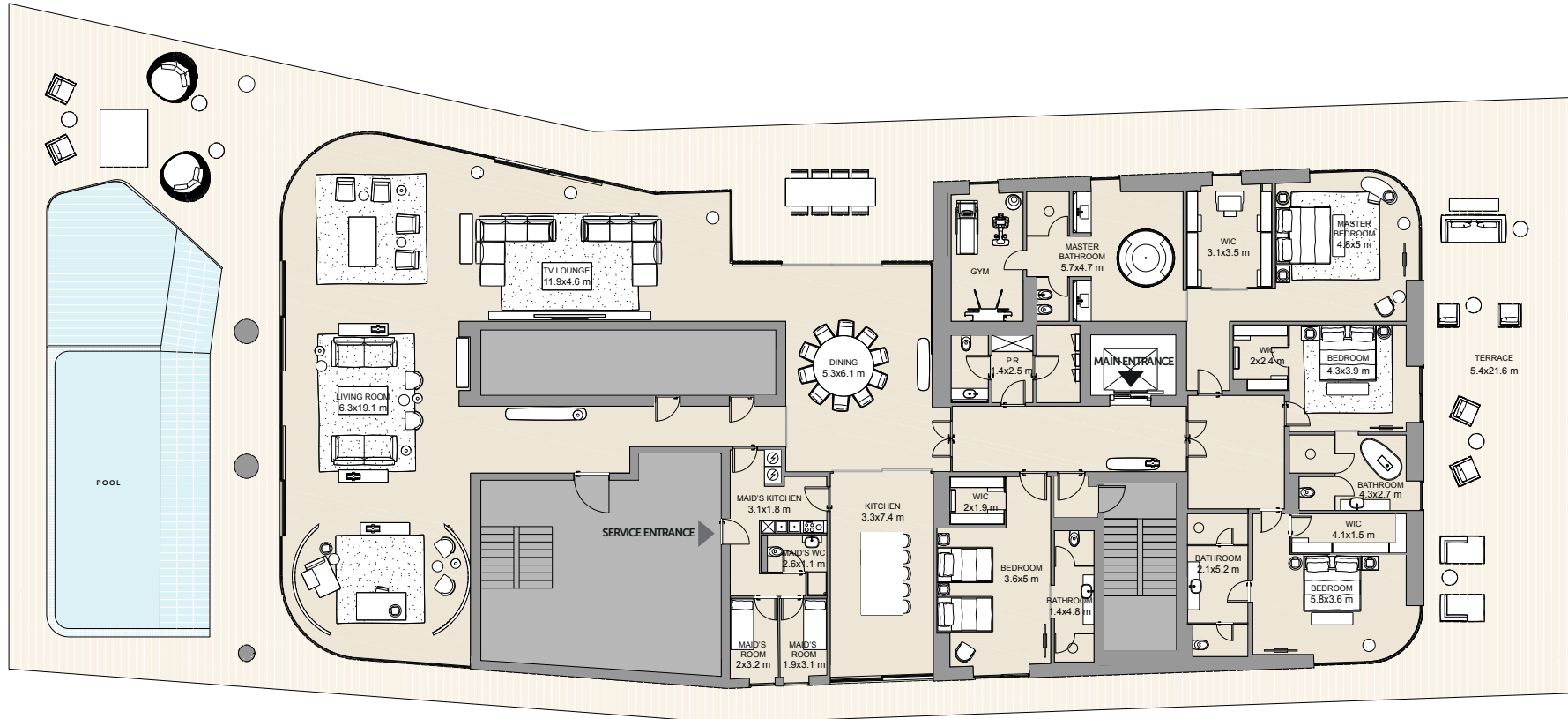
FLOOR SHAPE
